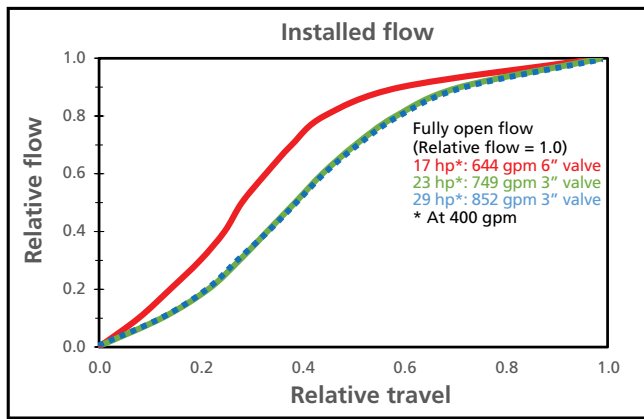
Figure 6. Control valve installed gain analysis helps balance pumping energy and process controllability. Segment valve graphic courtesy of Neles
