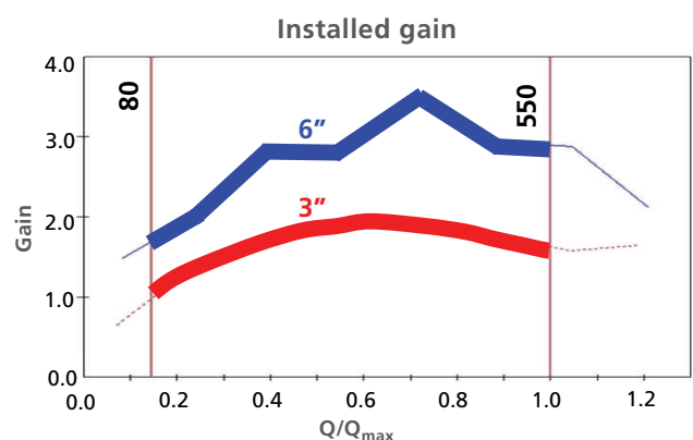
Figure 1. Control valve installed flow and installed gain characteristics comparing a properly sized 3-inch valve and an oversized 6-inch valve in the same system. Emphasis is added to show the portion of the graphs that fall within the user’s specified flow range between minimum and maximum required flow of 80 to 550 gpm.
