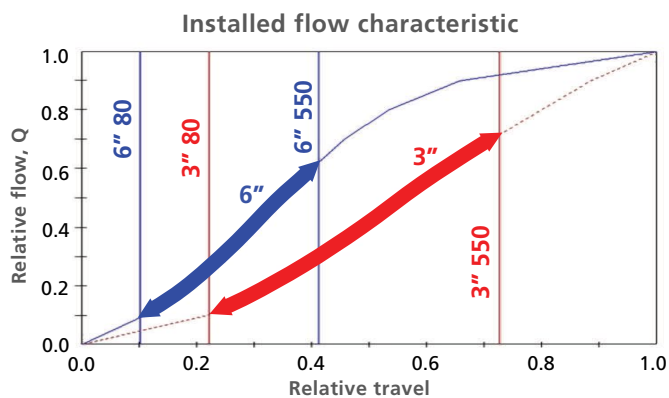
Figure 1. Control valve installed flow and installed gain characteristics comparing a properly sized 3-inch valve and an oversized 6-inch valve in the same system. Emphasis is added to show the portion of the graphs that fall within the user’s specified flow range between minimum and maximum required flow of 80 to 550 gpm.
