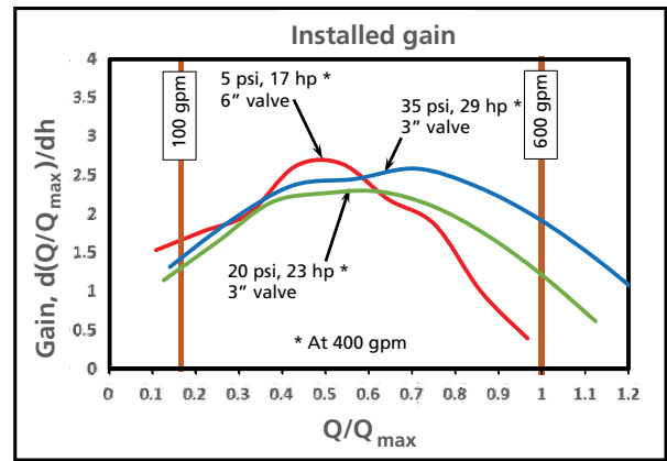
Figure 6. Control valve installed gain analysis helps balance pumping energy and process controllability. Segment valve graphic courtesy of Neles
